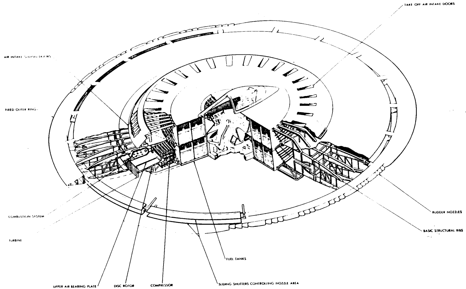
Fig. 4 Section Cutaway of Research Aircraft (Radial Flow Engine)
