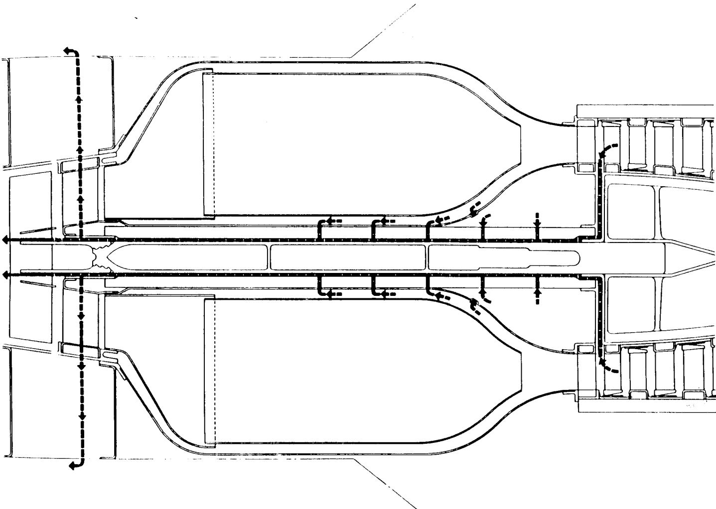
Fig. 12 Cross-Section Showing Bearing Airflow
